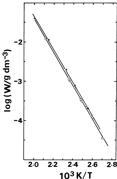
Fig. 2. Plot of \log (W/g \text{ dm}^{-3}) versus 1/T . \circ : \text{H}_2 -sulfur vapor system, \blacktriangle : \text{N}_2 -sulfur vapor system.
